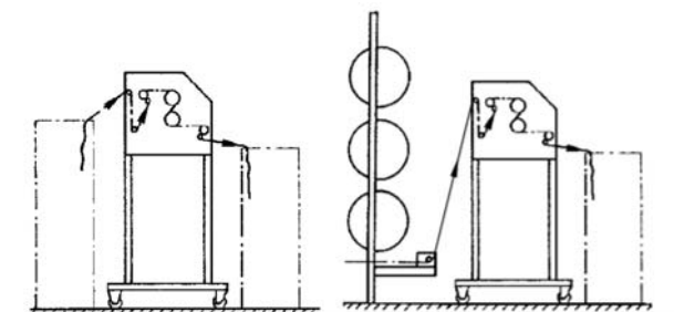
MÜTHERM 2/450: free-standing, mobile unit and fitted unit
