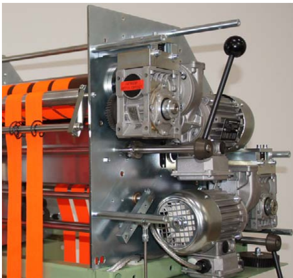
Separately controlled motors for infeed and outlet roller
